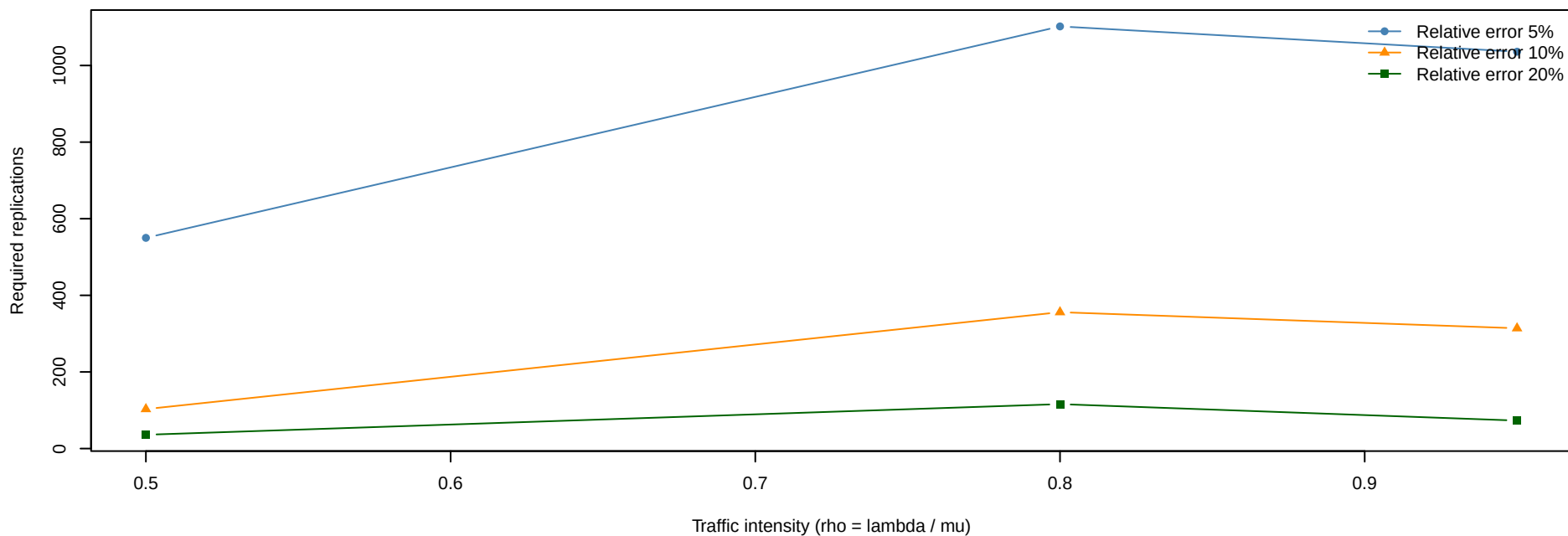
Required replications; 1000 delays per replication
